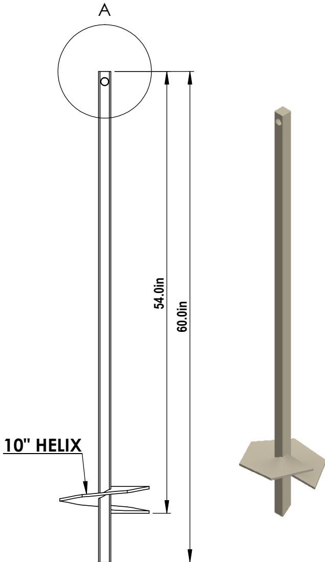
1 1.5" RCS SINGLE HELIX 1" = 1' 0"
